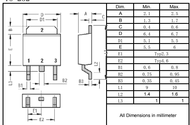
T0-252
